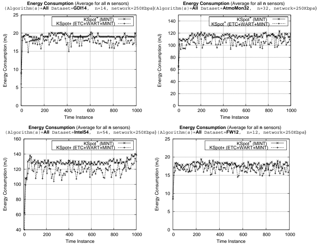
Figure 8: Energy consumption for KSpot + (MINT) and KSpot + (ETC+WART+MINT) using the TelosB energy model.
