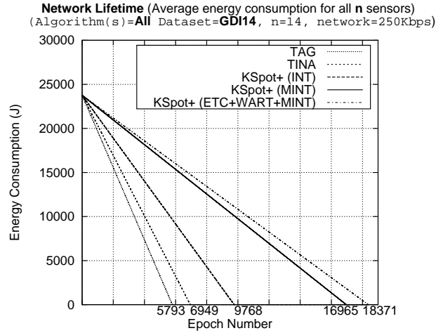
Figure 9: Network lifetime for all algorithms.
